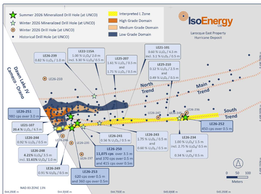
Figure 2 – Hurricane South Trend mineralized drill hole locations on the Larocque East project, including summer program holes LE26-250, 251, 252, and 253 completed to date
